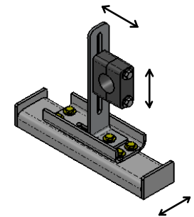
BOLT-ON PIPE MOUNT ASSY
